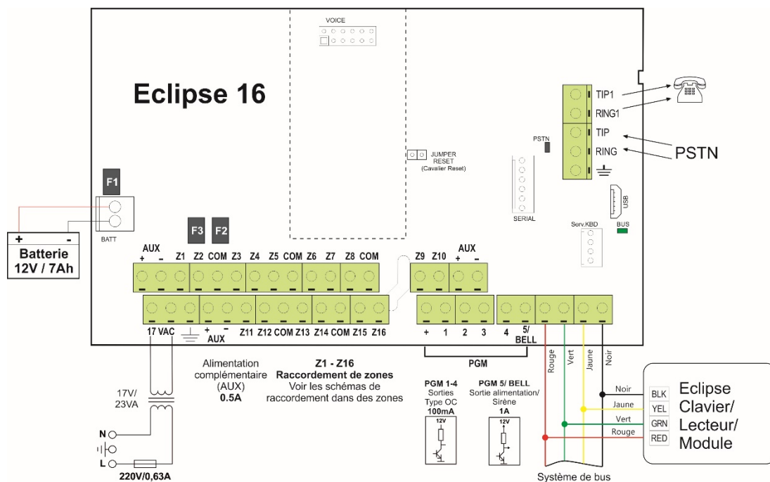
Figure 6. Centrale ECLIPSE 16
