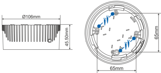
Disassembling
