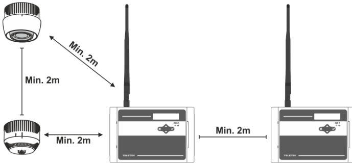
Wireless fire base – Dimensions and mounting
