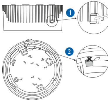
Assembling
